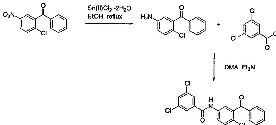
Scheme XI
